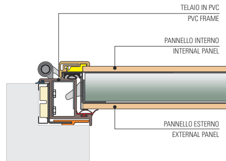
NODO TELAILO SYNERGY-OUT SYNERGY-OUT FRAME NODE
